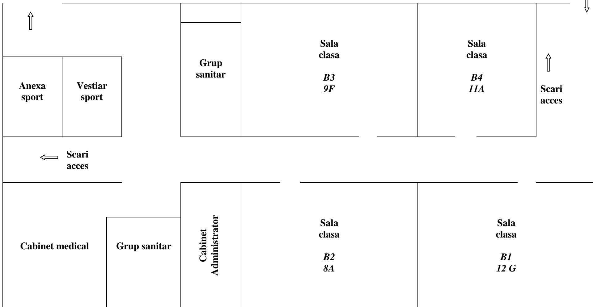
CORPUL B PLAN PARTER
